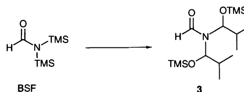
Scheme 1 Reagents and conditions: BSA (1 equiv.), room temp., then TMSOTf, CCl 4 ; and finally Pr i CHO (4 equiv.), room temp., 3 h (99%)
