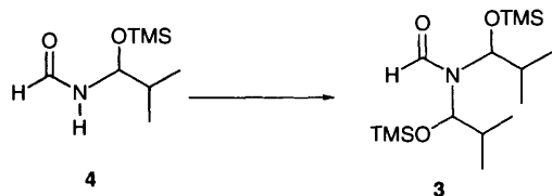
Scheme 2 Reagents and conditions: BSA (3 equiv.), room temp., 4 h; then Pr t CHO (2.9 equiv.), TMSOTf (cat.), room temp., 0.25 h (100%)
